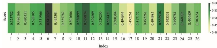
Fig 3. Graph of similarity indices from the TOPSIS technique, according to expert evaluations in the questionnaire Based on the findings from the questionnaire and TOPSIS technique, the category of indicators related to "renovation" has the greatest impact on improving the quality of urban facades in the studied sample.
